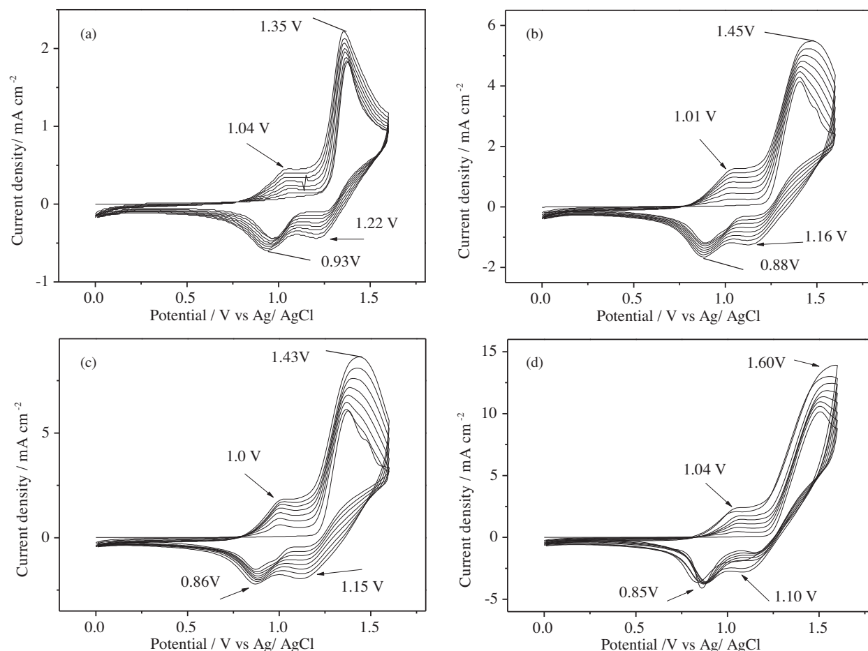
Figure 4. Cyclic voltammetry of MCzCTB was performed on a glassy carbon electrode (GCE) in various initial monomer concentrations in 1 M H 2 SO 4 solution, a) [MCzCTB] 0 = 1 mM, b) [MCzCTB] 0 = 3 mM, c) [MCzCTB] 0 = 5 mM, d) [MCzCTB] 0 = 10 mM, 8 cycle, scan rate: 100 mV s -1 . Potential range: 0.0 V–1.6 V.
