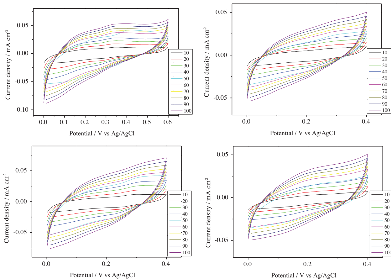
Figure 5. Cyclic voltammety of MCzCTB was performed in monomer-free solution on a glassy carbon electrode (GCE) in various initial monomer concentrations in 1 M \text{H}_2\text{SO}_4 solution, a) [\text{MCzCTB}]_0 = 1 mM. Potential range: 0.0 V–0.6 V, b) [\text{MCzCTB}]_0 = 3 mM. Potential range: 0.0 V–0.4 V, c) [\text{MCzCTB}]_0 = 5 mM. Potential range: 0.0 V–0.4 V, d) [\text{MCzCTB}]_0 = 10 mM. Potential range: 0.0 V–0.4 V. Polymerization was performed by 8 cycles, scan rate: 10 \text{ mV s}^{-1} , scan rates were taken in monomer-free solution as 10, 20, 30, 40, 50, 60, 70, 80, 90, and 100 \text{ mV s}^{-1} .
