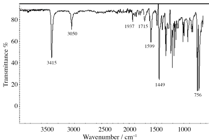
Figure 2. FTIR spectrum of MCzCTB.
