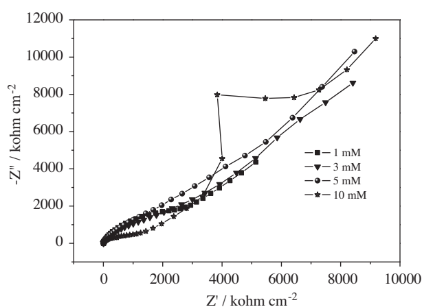
Figure 8. Nyquist plot of P(MCzCTB)/GCE in various initial monomer concentrations (1, 3, 5, and 10 mM). Experimental conditions are given in the following parameters, 8 cycles at a scan rate of 100 mV s -1 in 0.1 M NaClO 4 /CH 3 CN.
