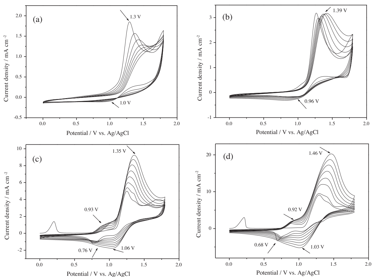
Figure 3. Cyclic voltammetry of MCzCTB was performed on a glassy carbon electrode (GCE) in various initial monomer concentrations in 0.1 M NaClO_4/CH_3CN , a ) [MCzCTB]_0 = 1 mM ( Q = 5.90 mC), b ) [MCzCTB]_0 = 3 mM ( Q = 9.86 mC), c ) [MCzCTB]_0 = 5 mM ( Q = 20.14 mC), d ) [MCzCTB]_0 = 10 mM ( Q = 43.28 mC). 8 cycles, scan rate: 100 mV s^{-1} . Potential range: 0.0 V– 1.8 V.
