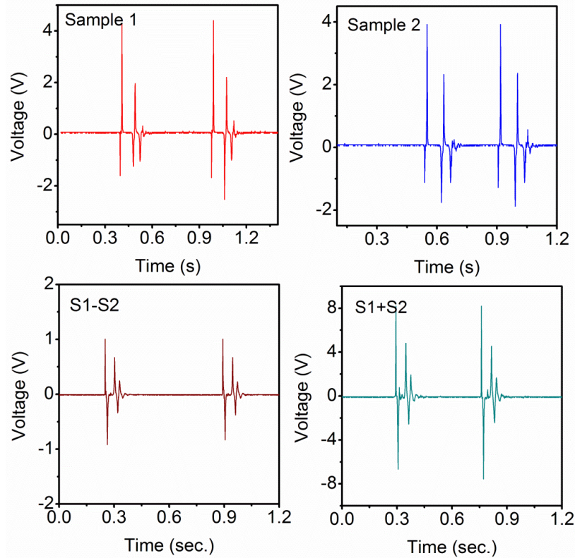
Fig. 7: Voltage response of two samples (S1, S2) and the superposition voltage output with additive effect and negating effect.
