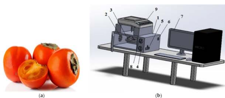
Figure 1. (a) Trabzon persimmon, (b) Microwave Drying System (1: Microwave oven, 2: Ventilation holes, 3: Tray, 4: Timer, 5: Magnetron, 6: Fan; 7: Computer, 8: Power switch, 9: Scales).
