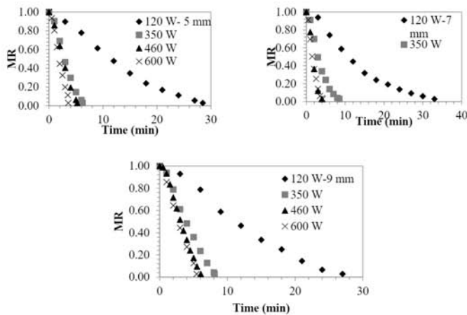
Figure 2. Changes in the moisture content based on time of the persimmons dried in varying microwave powers and varying slice thicknesses.
