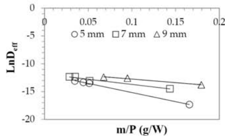
Figure 3. Microwave powers effect on effective diffusion coefficient.
