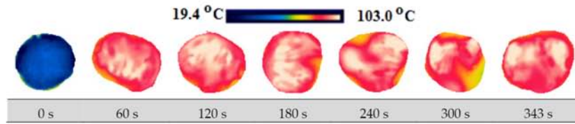
Figure 21. Thermal images.
