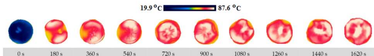
Figure 10. Thermal images of persimmon with 5 mm at 120 W.
