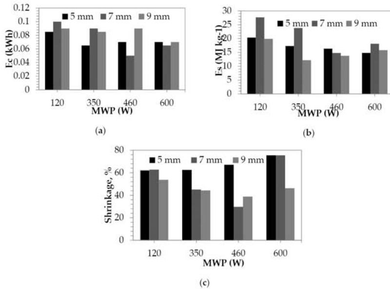
Figure 5. (a) Energy consumption values of the microwave dryer, (b) the specific energy consumption of the persimmon at varying powers and slices during the drying, (c) percentage shrinking of the persimmon during the drying.
