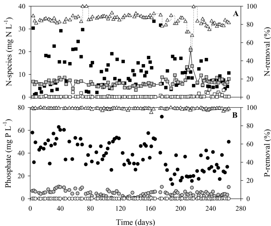
Fig. 1. Experimental profiles during the 261 d of operation of the A 2 /O plant. A) Ammonium concentration in the influent (■) and effluent (□), nitrate concentration in the effluent (●) and N-removal efficiency (Δ). B) Phosphorus concentration in the anaerobic reactor (●), anoxic reactor (○) and effluent (○) and P-removal efficiency (Δ).
