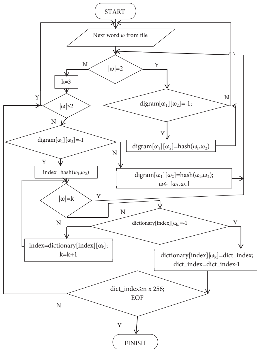
Figure 3. Dictionary insertion.
