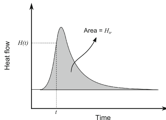
Fig. 5 Schematic description of a DSC scan for the heat generated during curing or crystallization. H(t) is the heat flow until the time t , H_{tr} is the total heat flow
