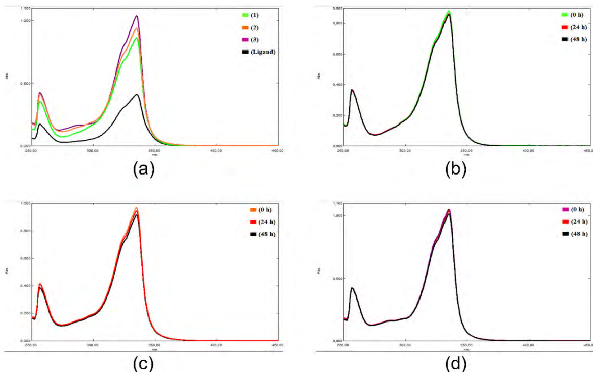
Figure 4. (a) UV-Vis spectra of bismuth(III) halide complexes and the free ligand in DMSO ( 10^{-3} M). (b) UV-Vis spectra of 1 for 0 h, 24 h and 48 h; (c) UV-Vis spectra of 2 for 0 h, 24 h and 48 h; (d) UV-Vis spectra of 3 for 0 h, 24 h and 48 h.
