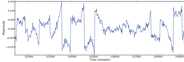
Fig. 10. Filtered EOG data without the drift and high frequency noise.
