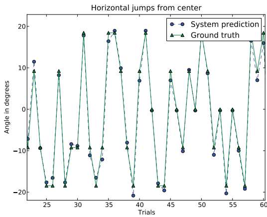
Fig. 15. The jumps between the center and the target provided by the system and the actual ones are quite similar for the horizontal axis.
