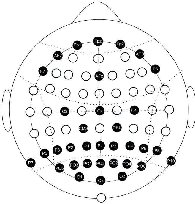
Fig. 3. Electrode positioning for EEG measurement: 32 electrodes positioned mainly on the parieto-occipital area as this is where the relevant alpha modulations for spatial covert attention are expected, and some others to look at artifacts and to offer the possibility to apply certain spatial filters.
