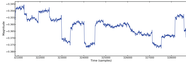
Fig. 9. EOG data is noisy and drifts over time.
