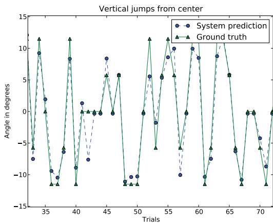
Fig. 16. The predictions of the system are quite less good than for the horizontal jumps.
