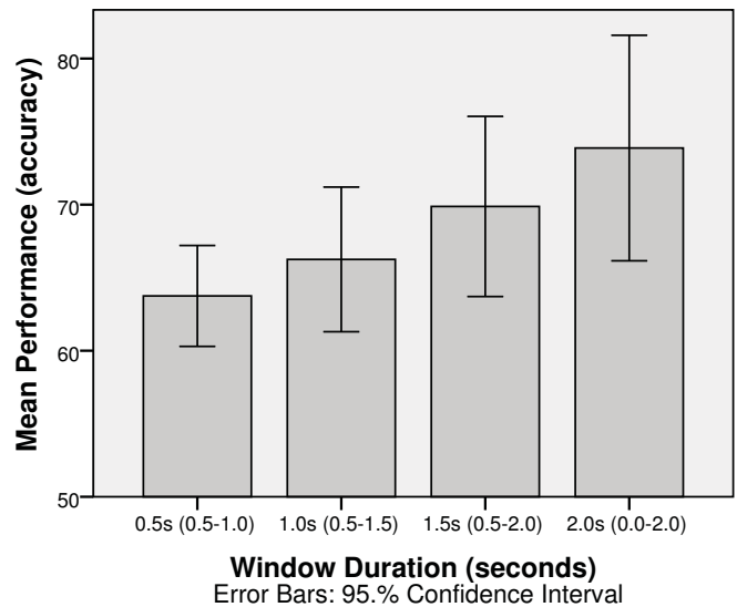
Fig. 7. Two-class covert attention performance for different window sizes, averaged over 6 participants. It shows an incremental increase for longer windows.
